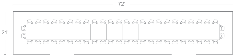
BRIDGING, 52 SEATS (scale reduced) Put some of your Summits between two fixed tables with WallGoldfinger's exclusive bridge design. Leave the Summits in place for a large meeting. Remove the Summits and engage an operable wall to create two meeting spaces.
